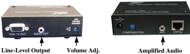
Figure 3.2 – Front and rear panels of URA-VOL
